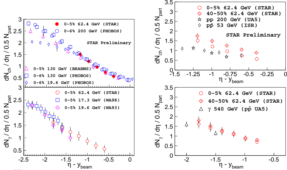
Figure 3. \frac{dN}{d\eta} for charged particles and photons [2] for various collision systems : (left) at different \sqrt{s_{NN}} and (right) for various event centrality classes at \sqrt{s_{NN}} = 62.4 GeV.
